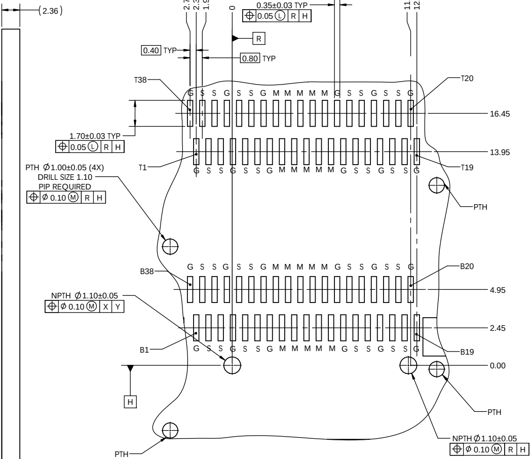
DETAIL B SCALE 8 : 1
