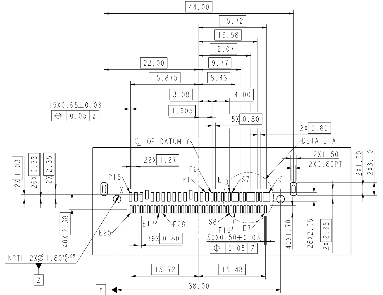
RECOMMENDED PCB LAYOUT (TOP VIEW) GENERAL TOLERANCE ±0.05 (PCB THICKNESS: 3.0MM)
