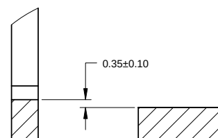
DETAIL B SCALE 6 : 1
