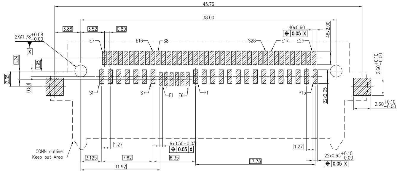
RECOMMENDED PCB LAYOUT(TOP VIEW) GENERAL TOLERANCE \pm 0.05\text{mm} (PCB THICKNESS: 3.0mm)
