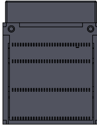
V62-CDZ01-0400X0T (WITHOUT SOLDER RING FOR SINGLE SIDE MOUNTING)
