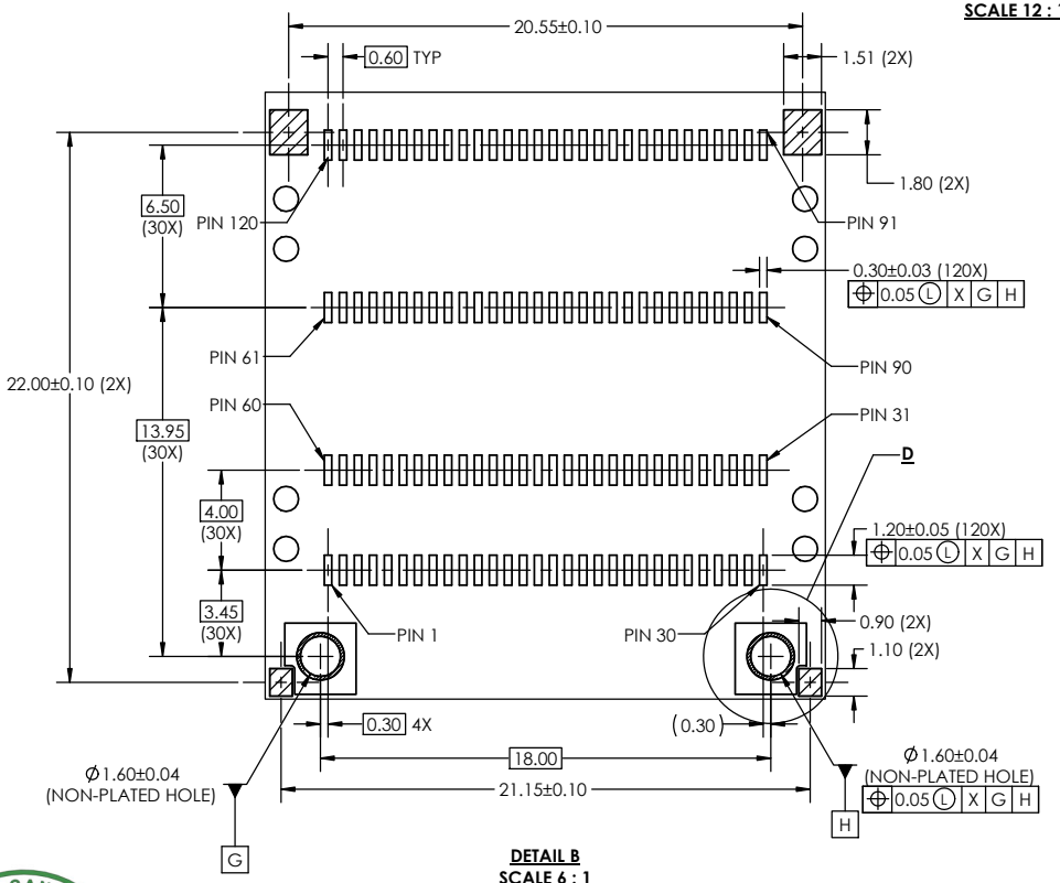
PADS FOR SOLDER RINGS (2 PLCS) DETAIL D SCALE 12 : 1
