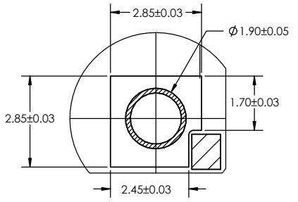
PADS FOR SOLDER RINGS (2 PLCS) DETAIL D SCALE 12 : 1
