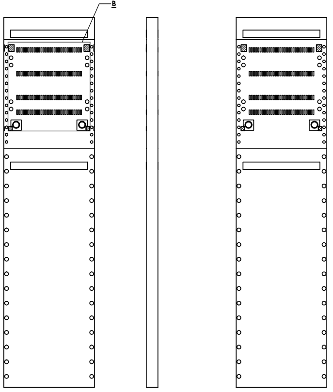
RECOMMENDED PCB LAYOUT FOR BELLY TO BELLY MOUNTING
